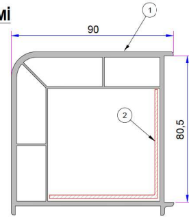
1. 90° Köşe Profili P.A.080.5100.600.0.00.19 2. Destek Sacı (60x60) 1,2mm - 34022 - 12306 1,5mm - 34022 - 15306 2 mm - 34022 - 20306
